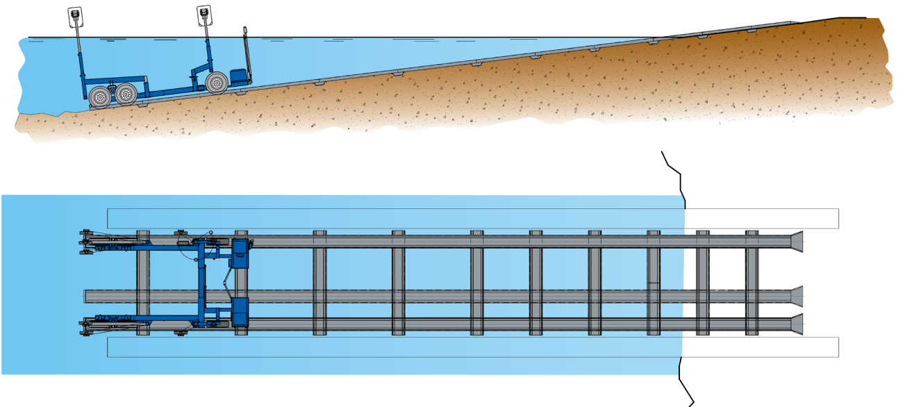
General sketch for a ramp made of U-shaped steel frames with three lanes for variable width and or different sized Sublift boat hoists.
